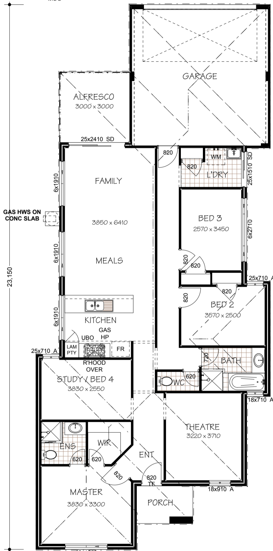
FLOOR PLAN
