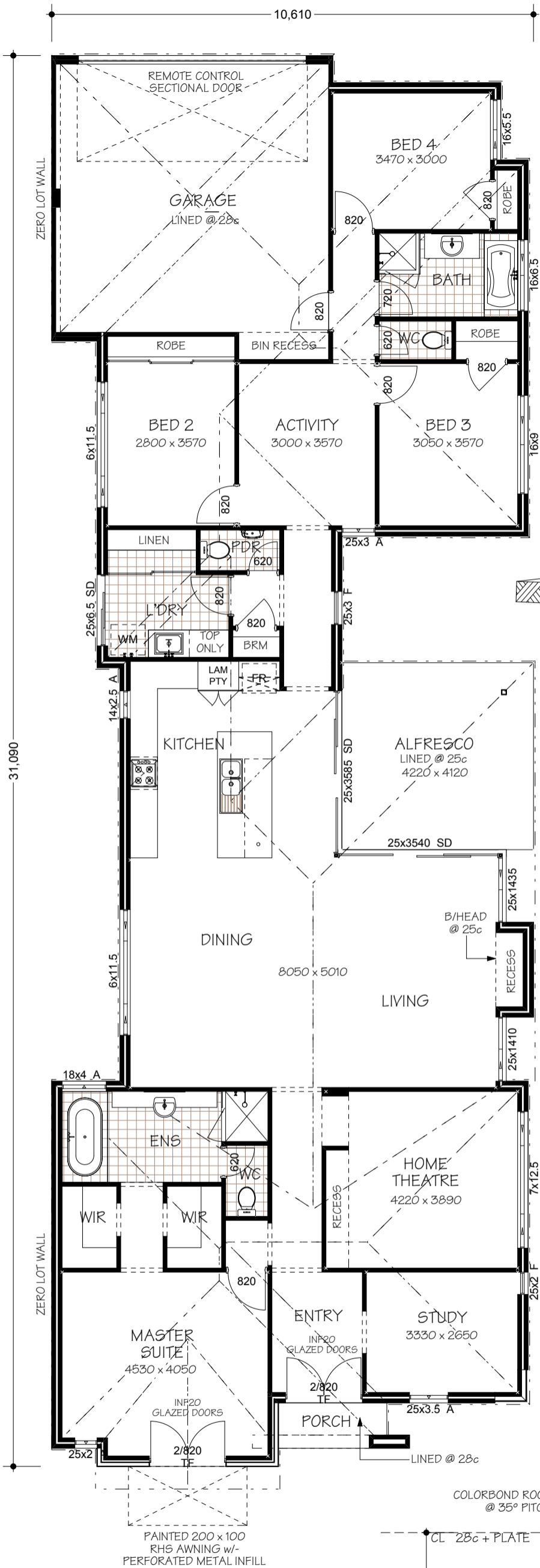
FLOOR PLAN 1:100
