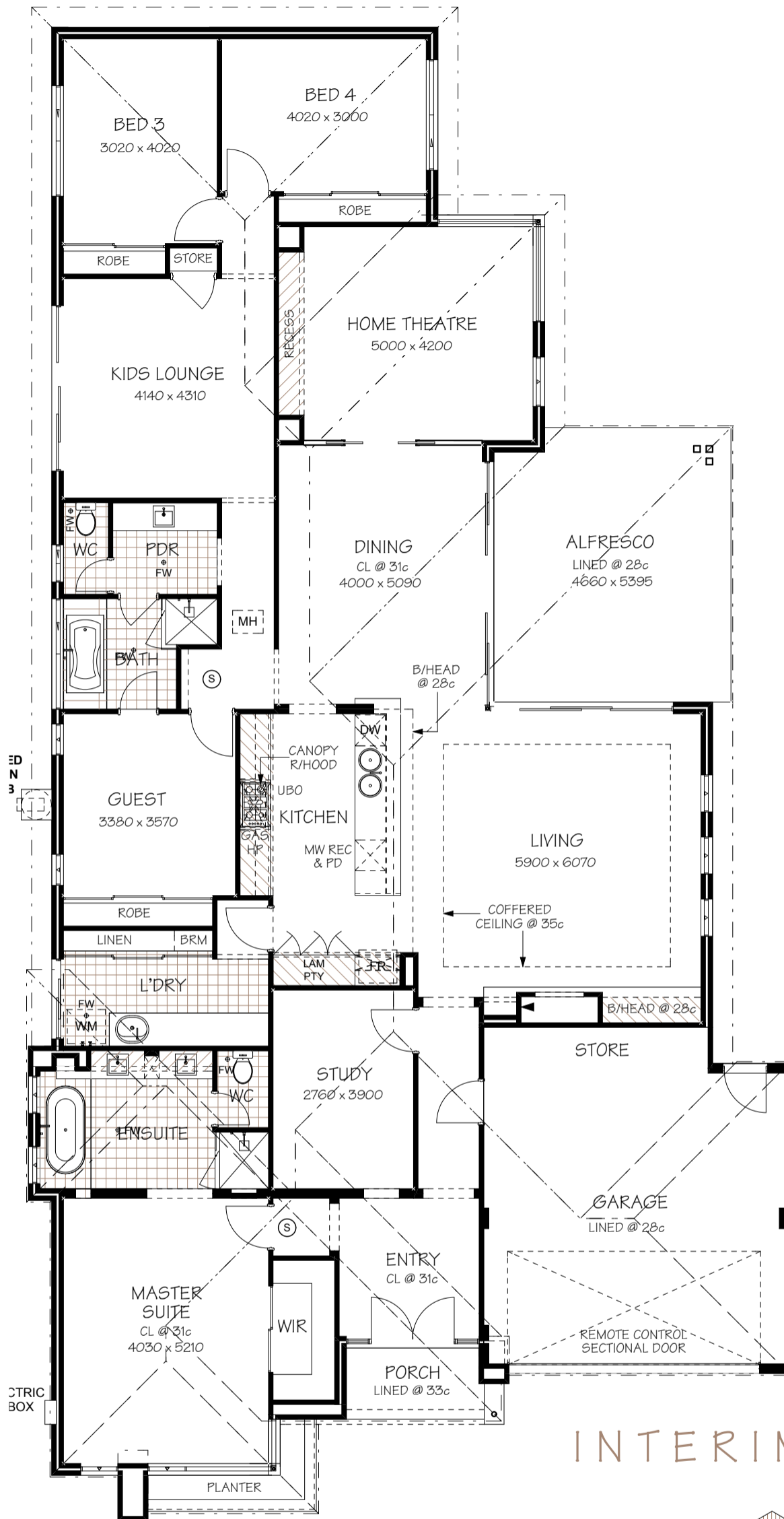
FLOOR PLAN 1:100
